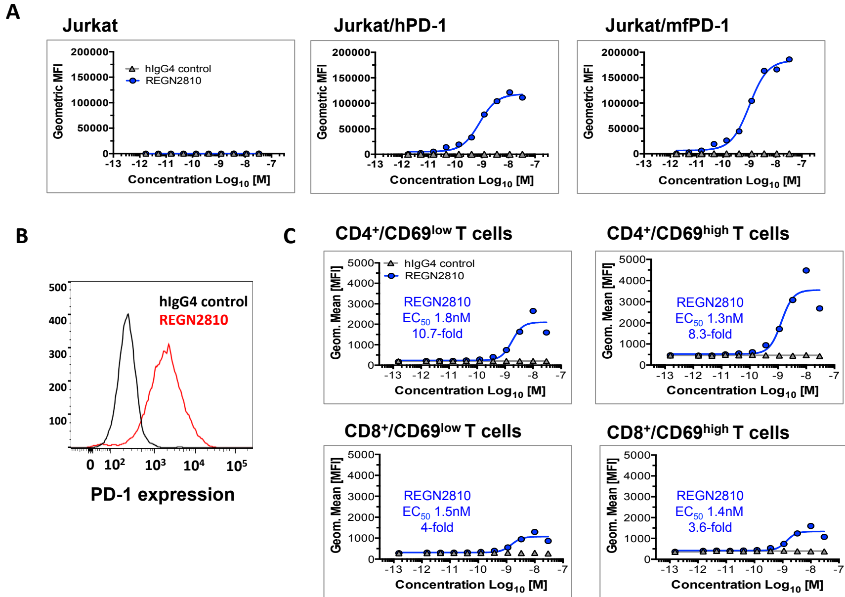
Figure S1. REGN2810 binds to PD-1 on engineered Jurkat cells and on activated human and cynomolgus monkey T cells.
