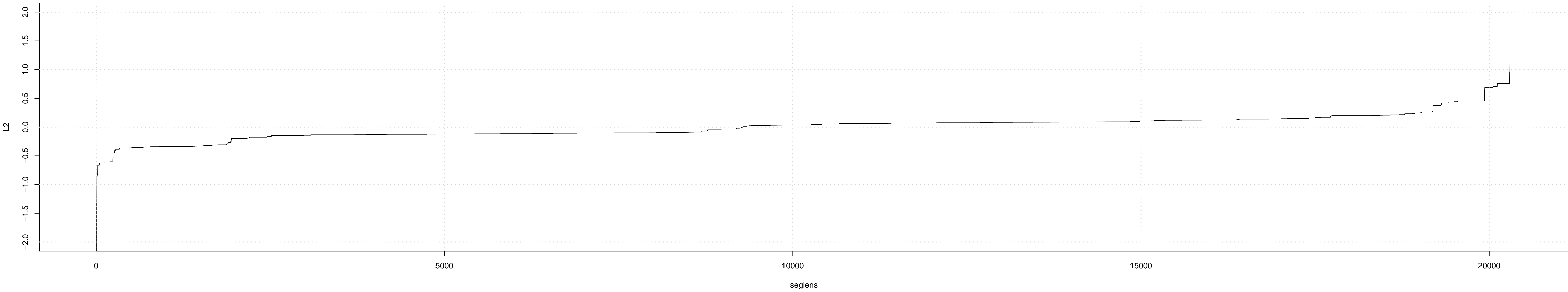
Supplementary Figure S2: D. Unscaled segments plot
