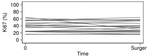
Control (part 1)
