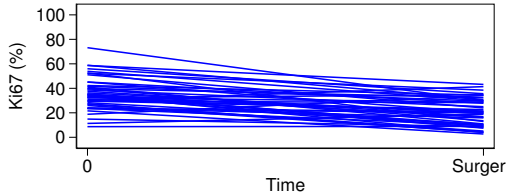
Lapatinib (part 1)
