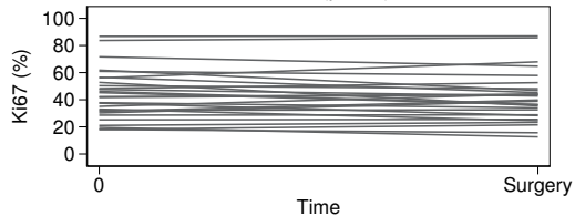
Control (part 2)
