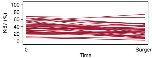
Trastuzumab (part 1)
