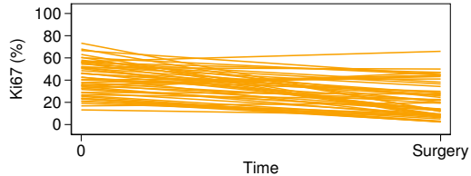
Combination (part 2)
