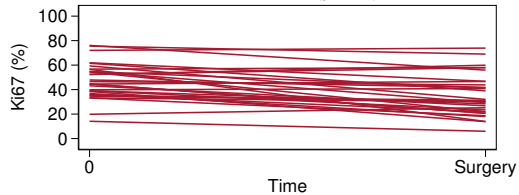
Trastuzumab (part 2)
