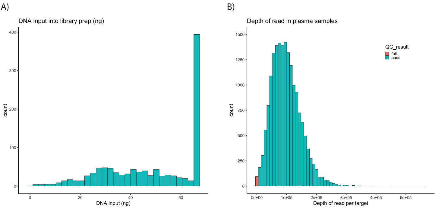
Supplementary Figure S1: Quality Control Metrics for cfDNA Sequencing by Signatera. A) DNA input for NGS libraries. Input was capped at 66 ng. B) Depth of Read (DoR) for each amplicon in plasma samples. Amplicons with DoR<5000 were counted as failed and excluded from further analyses.
