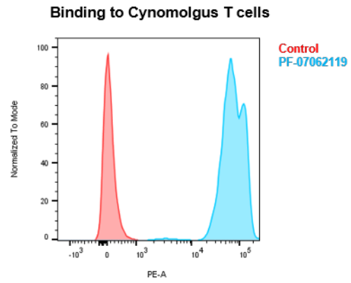
Figure S7. PF-07062119 binds to Cynomolgus Monkey T cells. Flow Cytometry analysis shows binding of PF-07062119 to cynomolgus monkey T cells.
