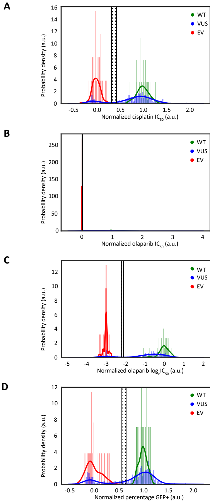
Figure S2: Functional assay data distribution curves. Distribution curves of the wild-type human BRCA1 (WT) and empty RMCE vector (EV) controls and BRCA1 VUS data in the (A) cisplatin, (B, C) olaparib (linear and logarithmic scale, respectively), and (D) DR-GFP HRR assays. Vertical solid and dotted black lines mark (from left to right) 0.99 and 0.95 probability of being deleterious and 0.95 and 0.99 probability of being neutral.
