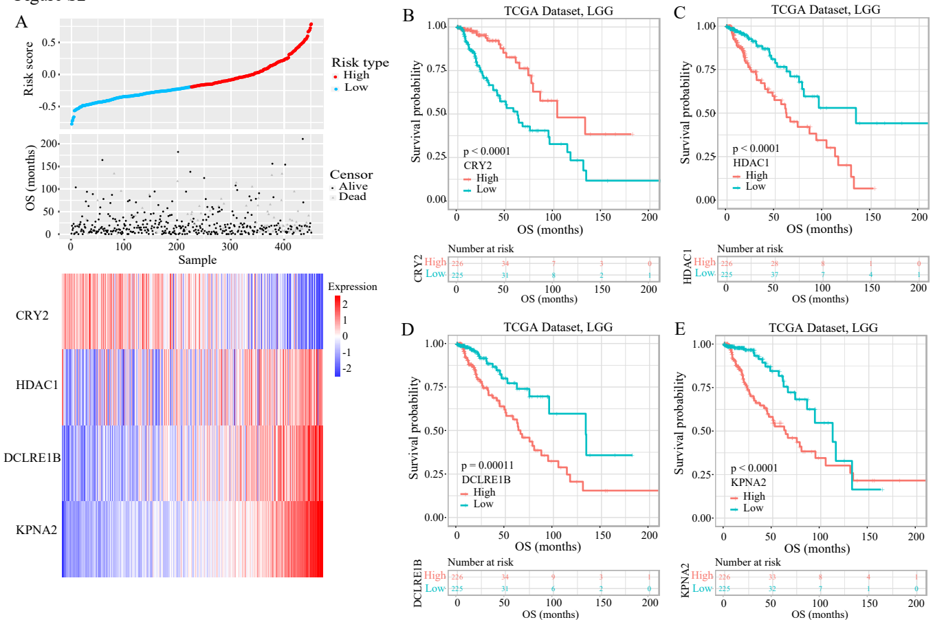
Figure S2 The association of four identified genes with risk score and patient survival in validation cohort. (A) From top to bottom are the risk score distribution, survival overview and heat map analysis of four genes. (B-E) Kaplan-Meier plot of OS according to the expression of CRY2, HDAC1, DCLRE1B and KPNA2.
