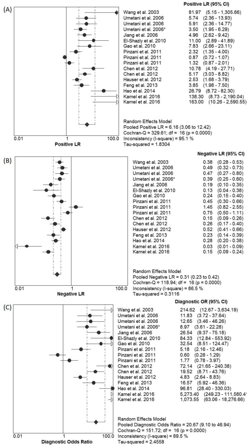
Supplemental Figure 1: Forest plots estimates of positive likelihood ratio (PLR) (A), negative likelihood ratio (NLR) (B) and diagnostic odds ratio (DOR) (C) for studies of cfDI in Group 1. Results with diamonds are pooled results, results with circles are single studies.
