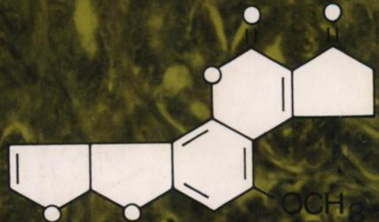
Aflatoxin B 1
