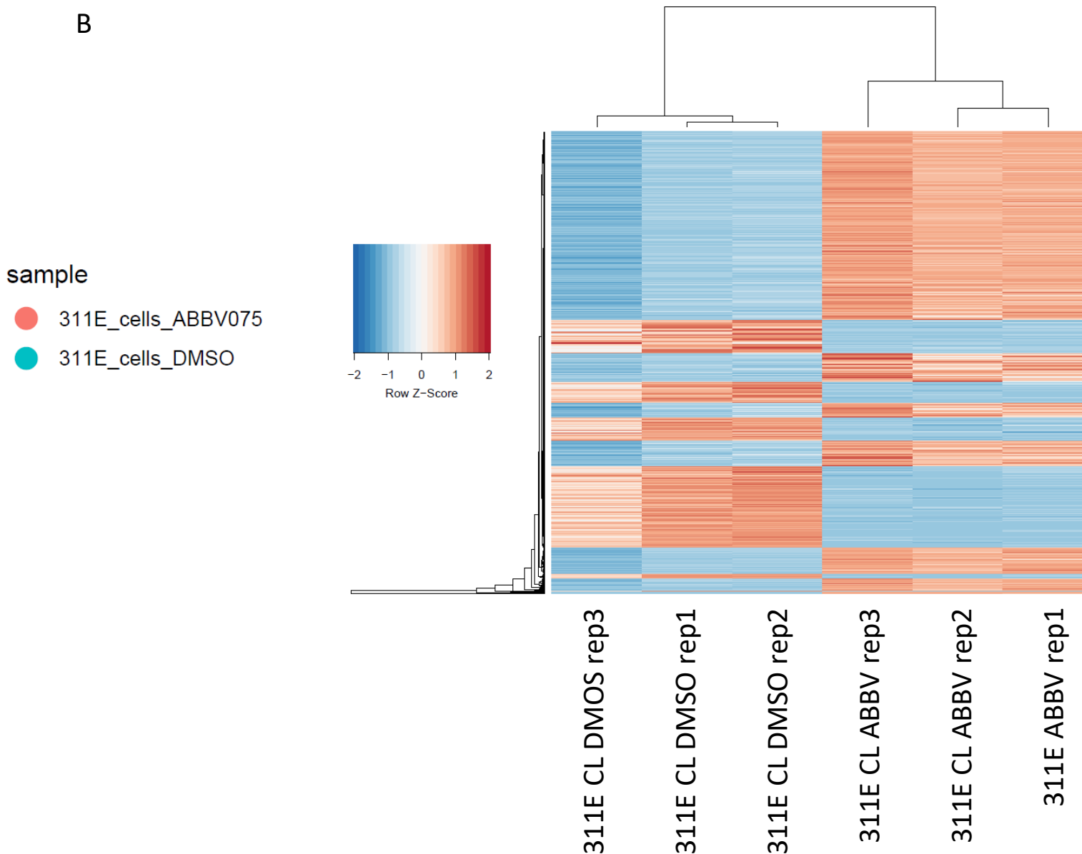
Supplementary Fig. S5. H3K27me3 and H3K27ac domains are mutually exclusive. A. Principal component analysis of RNAseq on the indicated samples based on all genes by variance. B. Heatmap of RNAseq results depicting all differentially expressed (DE) genes in 311E mNC cells treated with ABBV-075 (9nM) for 96h compared with those treated with DMSO. The treatment was done in biologic triplicate. ABBV, ABBV-075; CL, cell line.
