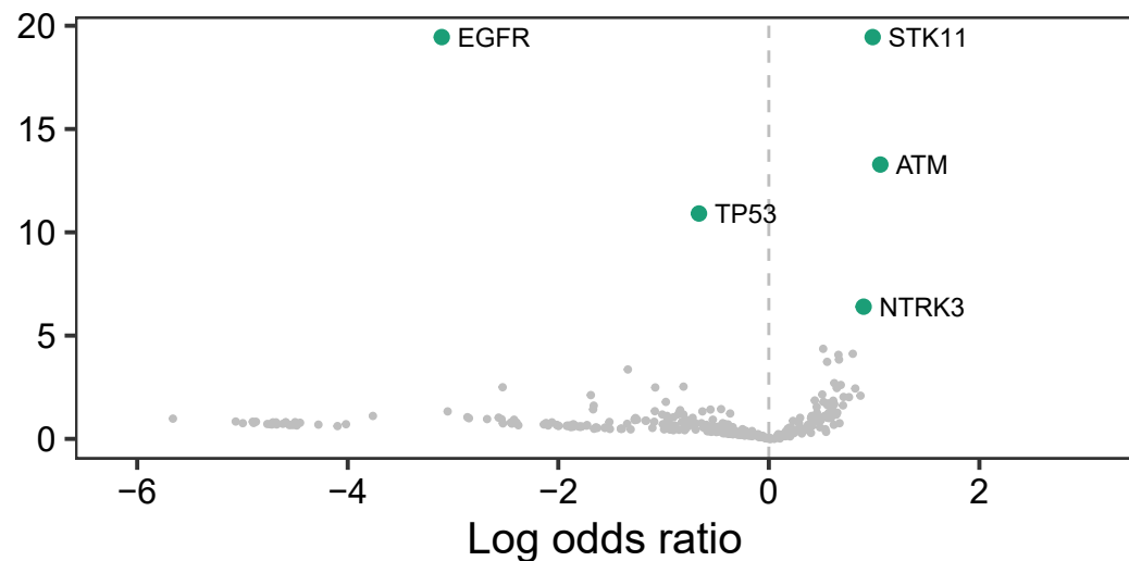
KRAS G12C
