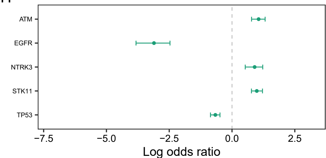
KRAS G12C
