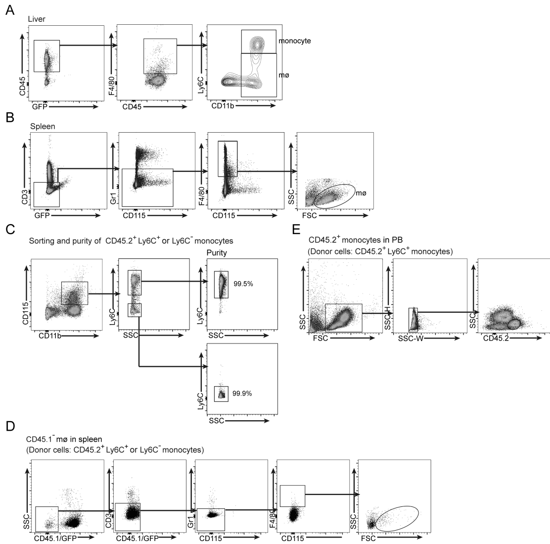
Figure S1. Gating strategy for macrophages in the liver and SP as well as monocytes/macrophages in the transplantation experiments at the steady state.
