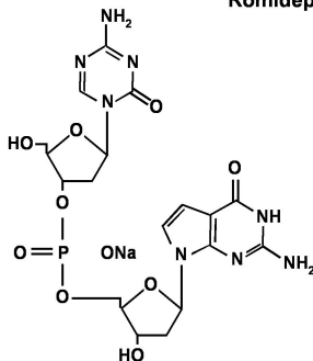
S110
