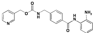
SDX-275
