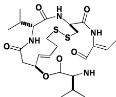
Romidepsin
