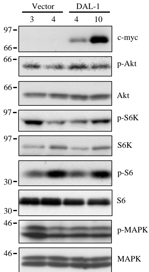
Supplemental Figure 3: Expression of DAL-1 does not activate other intracellular MAPK signaling pathways in IOMM-Lee cells. Lysates similar to those used in Figure 1A were analyzed by Western blot for activation of other signaling molecules. No reproducible changes in Akt, MAPK, S6, or S6-K activation (as represented by protein phosphorylation) were observed, when compared to total levels of each protein.
