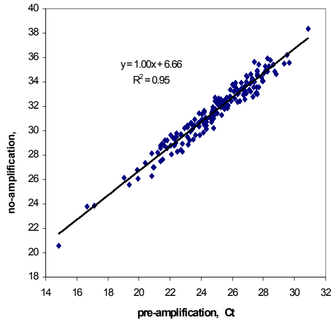
Supplemental Figure 1. The correlation between Ct values of unamplified cDNA (assayed by qRT-PCR) and post-amplification samples (using TLDA) was examined in seven RNA samples with sufficient amount available for both methods. 1 ug of RNA for no-amplification and 100ng of RNA for pre-amplification were used.
