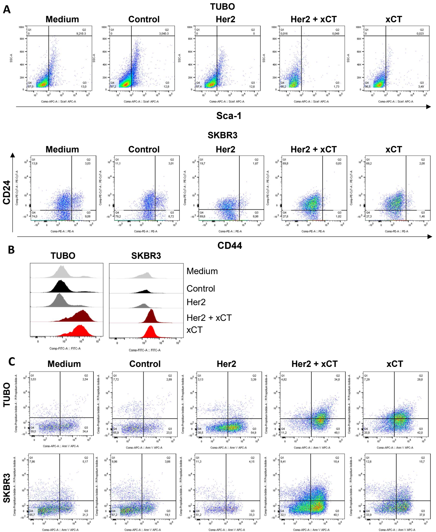
Supplementary Fig. S7. xCT antibodies induced CSC cell death. Representative FACS plots of Dissociated TUBO- or SKBR3-derived tumorspheres were incubated for 5 days with or without sera (1:50) from vaccinated mice, then analyzed by FACS. (A) Representative density plots of Sca1 and CD44/CD24 expression on TUBO and SKBR3 tumorspheres, respectively. (B) Representative histograms of DCF staining for intracellular ROS. (C) Representative Annexin-V/7-AAD density plots for apoptosis analysis. The same staining protocol and gating strategies were used for the analysis of ferroptosis. Representative results from 3 independent experiments.
