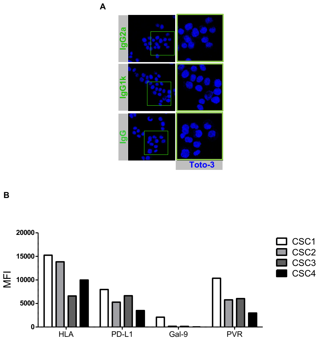
Supplementary Figure 2. CSCs characterization. (A) Negative controls for CD44, CD271, ABCB5, and CD166 antibodies on melanoma CSCs. Representative immunofluorescence analysis of IgG2a mouse monoclonal, IgG1k mouse monoclonal and goat IgG isotype controls on melanoma CSCs. Nuclei are stained with Toto-3 (blue). (B) Expression of NK cells immunomodulatory ligands on four melanoma CSC cell lines.
