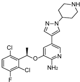
crizotinib
