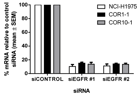
SI figure 8. (A) CO-1686 resistant clones COR 1-1 and COR 10-1 develop spindle-like morphology as compared to the parental NCI-H1975 cells (5x magnification). (B) EGFR expression as determined by qRT-PCR in NCI-H1975, COR1-1 and COR10-1 clones following siRNA knock-down 72-hours post-transfection.
