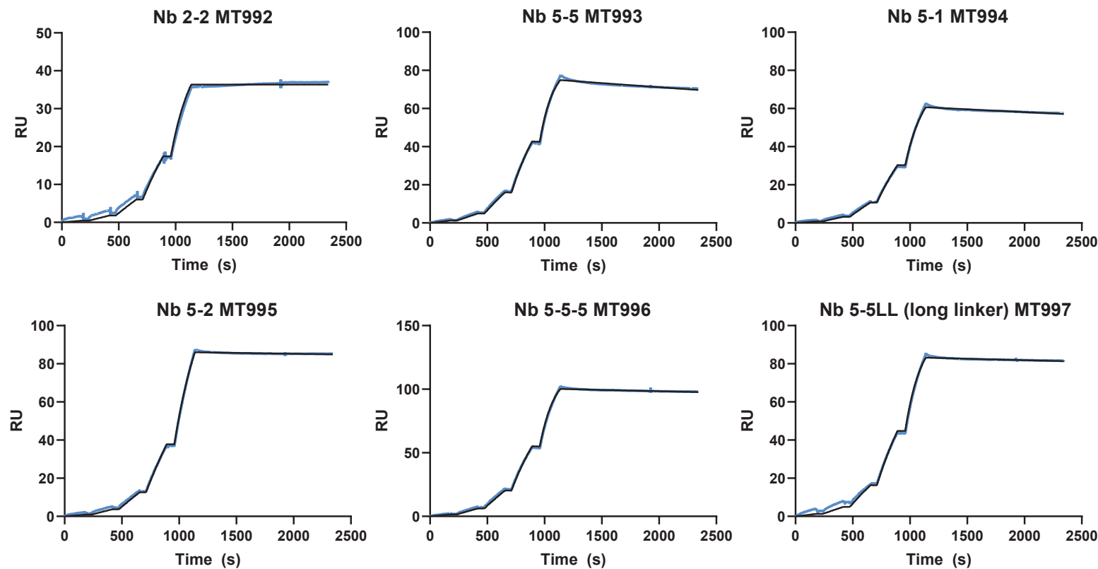
Supplementary Figure 13. Representative SPR sensorgrams of ORF1 monoclonal antibodies and “2nd Gen.” nanobody multimers. Single-cycle kinetics performed over immobilized ORF1, with (A) monoclonal antibodies or (B) nanobody multimers injected sequentially at 0.1, 0.3, 1, 3, and 10nM concentrations. Raw data (blue) and a 1:1 binding model fit (black) are plotted.
